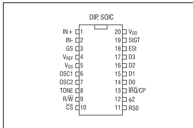
Figure 1 Pin Diagram
