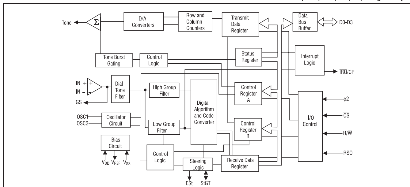
Figure 2 Block Diagram
