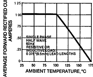
Fig. 5—FORWARD DERATING CURVE
