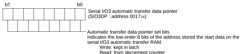
Fig. 37 Structure of serial I/O3 automatic transfer data pointer
