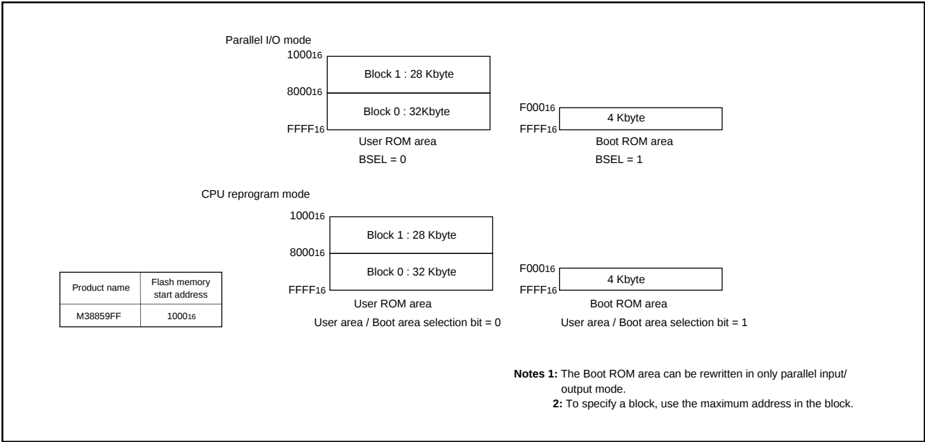
Fig. 72 Block diagram of flash memory version
