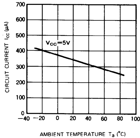
CIRCUIT CURRENT VS. AMBIENT TEMPERATURE (M51943B, M51944B)
