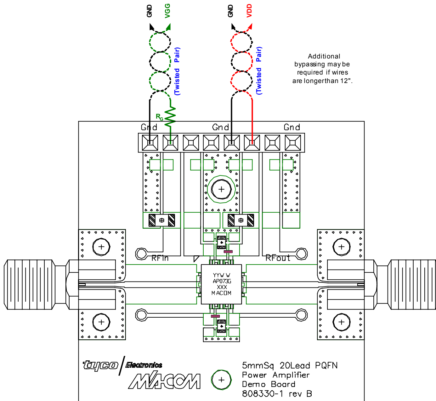
Figure 29. Demonstration Board P/N MAAP-000073-SMB003 (available upon request).
