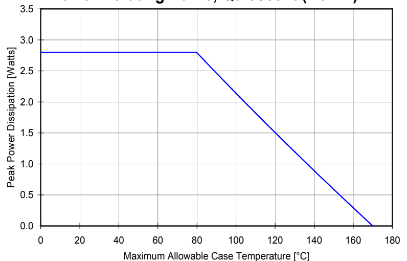
Power Derating Curve, Quiescent (No RF)
