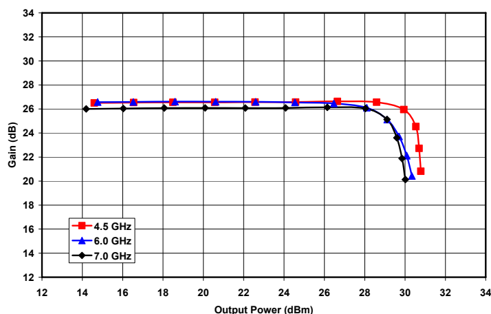
Figure 10. Gain vs. Output Power and Frequency at VD = 8V and IDQ = 0.33A
