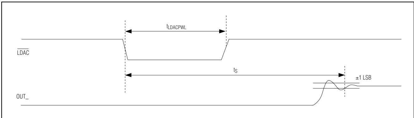
Figure 14. \overline{\text{LDAC}} Functionality
