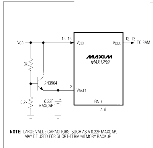
Figure 3. Using a MAXCAP as a Backup Battery
