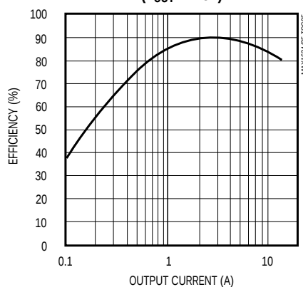
MAX1624 EFFICIENCY vs. OUTPUT CURRENT ( V_{OUT} = 2.5\text{V} )
