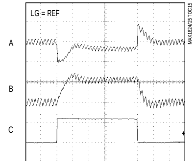
MAX1624 LOAD-TRANSIENT RESPONSE (WITHOUT GLITCHCATCHER) (3.5V)
