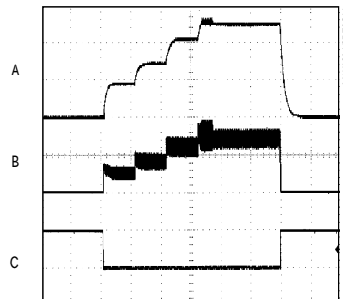
MAX1624 STARTUP AND STANDBY RESPONSE
