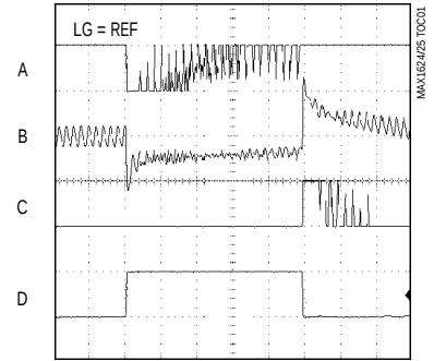
MAX1624 LOAD-TRANSIENT RESPONSE DETAIL (WITH GLITCHCATCHER) (1.1V)
