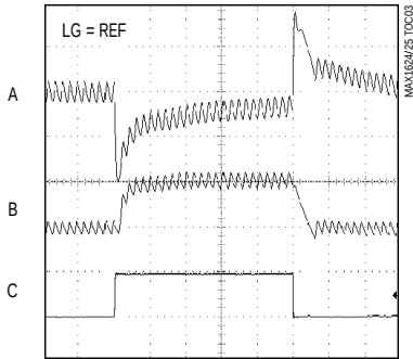
MAX1624 LOAD-TRANSIENT RESPONSE (WITHOUT GLITCHCATCHER) (1.1V)
