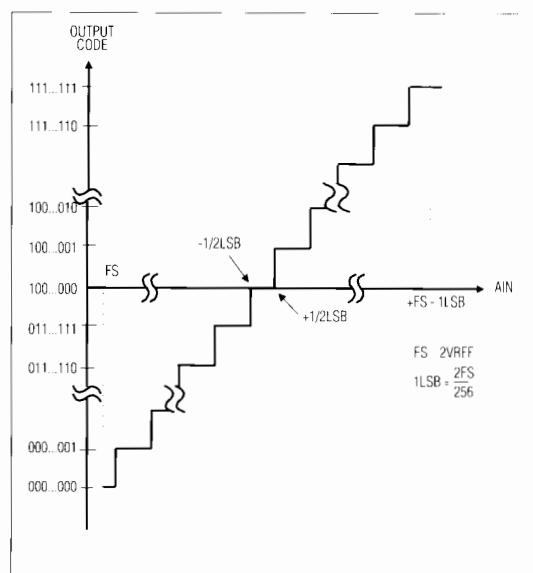
Figure 18b. Nominal Transfer Characteristic for Bipolar Operation
