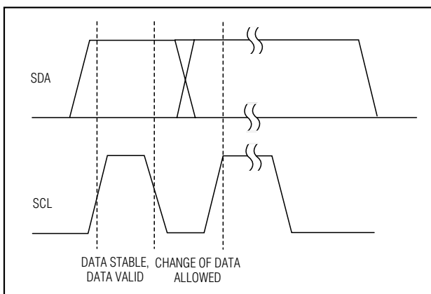
Figure 4. Bit Transfer
