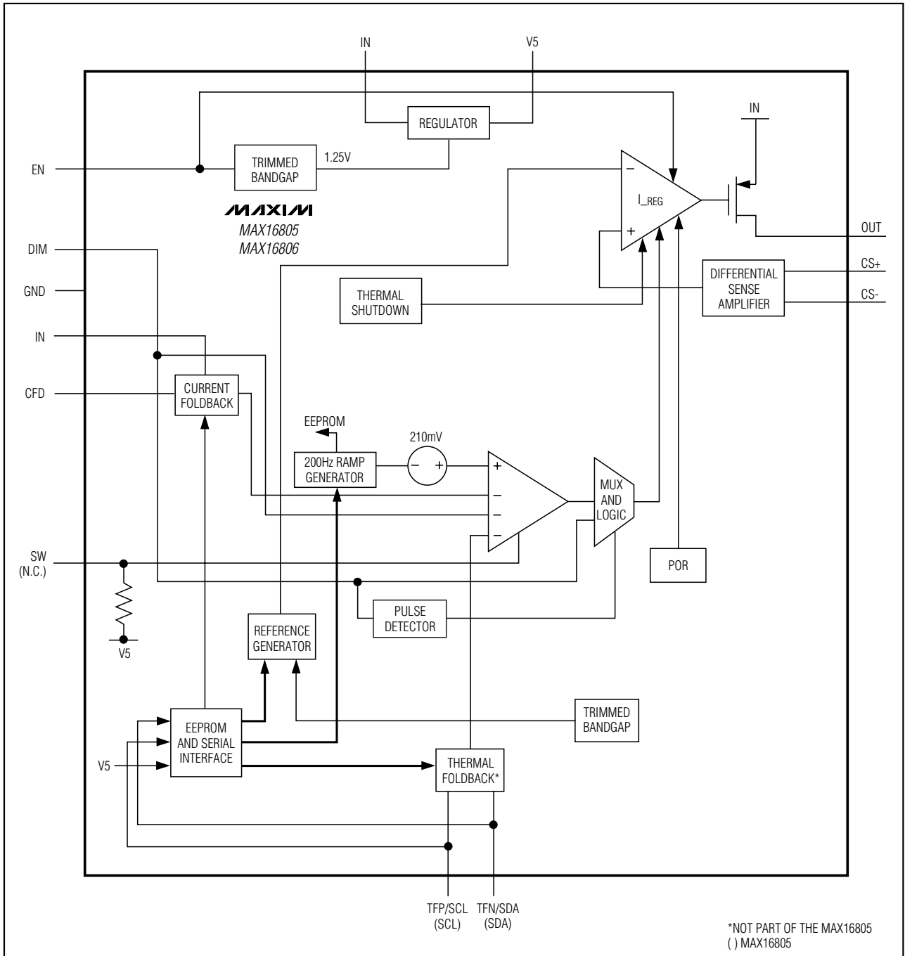
Functional Diagram
