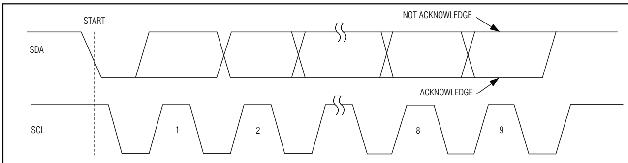
Figure 5. Acknowledge
