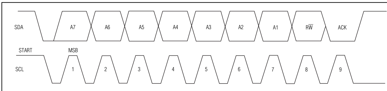
Figure 6. Slave Address
