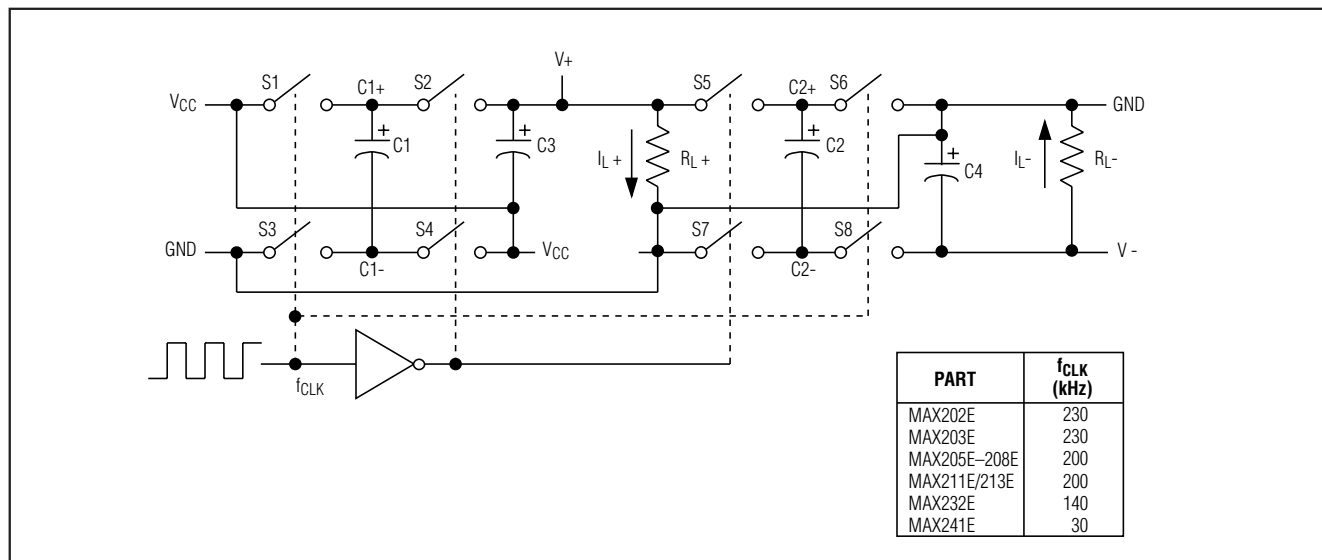
Figure 4. Charge-Pump Diagram
