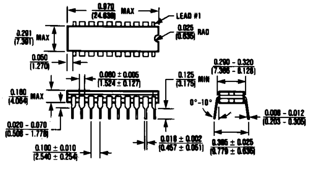
20 Lead Cerdip
