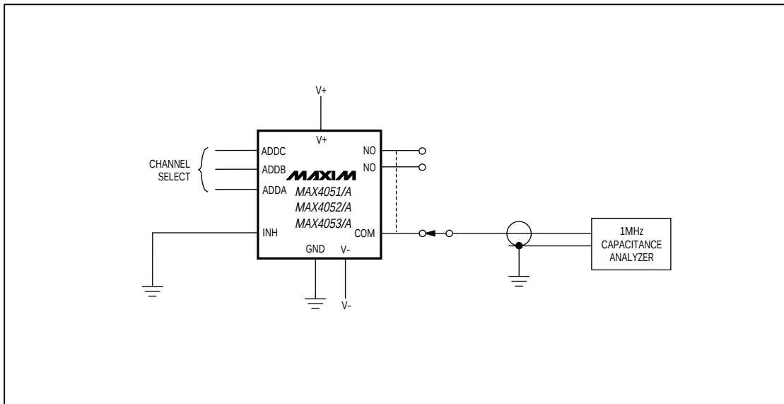
Figure 7. NO/COM Capacitance
