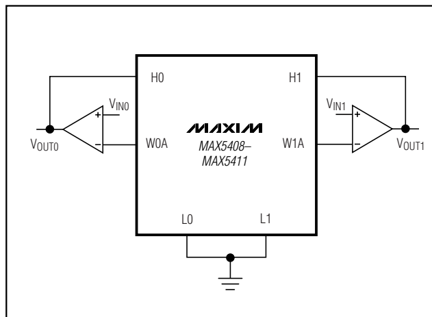
Figure 6. Gain Control
