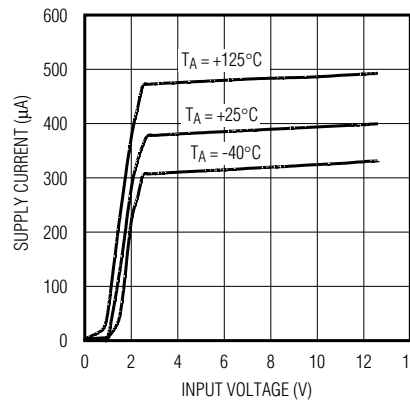
MAX6126_21 SUPPLY CURRENT vs. INPUT VOLTAGE
