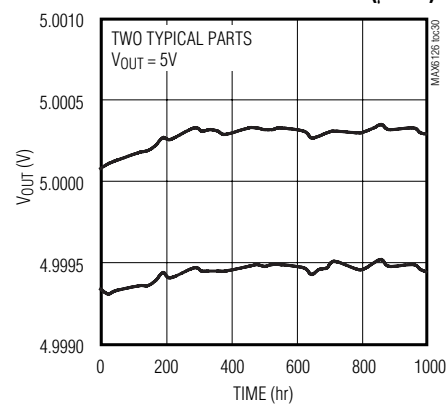
MAX6126B_50 LONG-TERM STABILITY vs. TIME ( \mu MAX)
