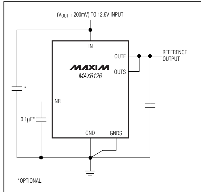
Figure 1. Noise-Reduction Capacitor
