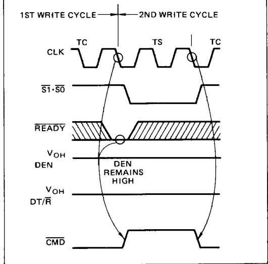
Fig. 8 – WRITE-WRITE BUS CYCLES WITH MB = 0
