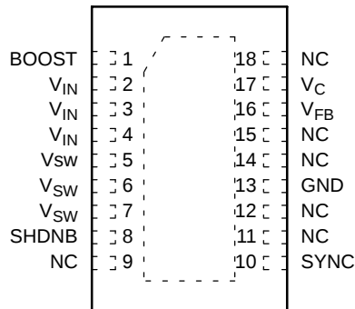
18-Lead DFN
