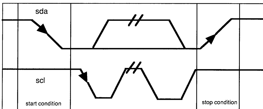
Figure 17. Start/Stop conditions
