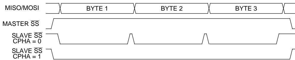
Figure 16-5. CPHA/SS Timing
