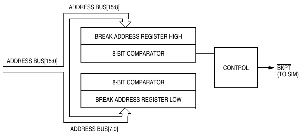
Figure 15-2. Break Module Block Diagram
