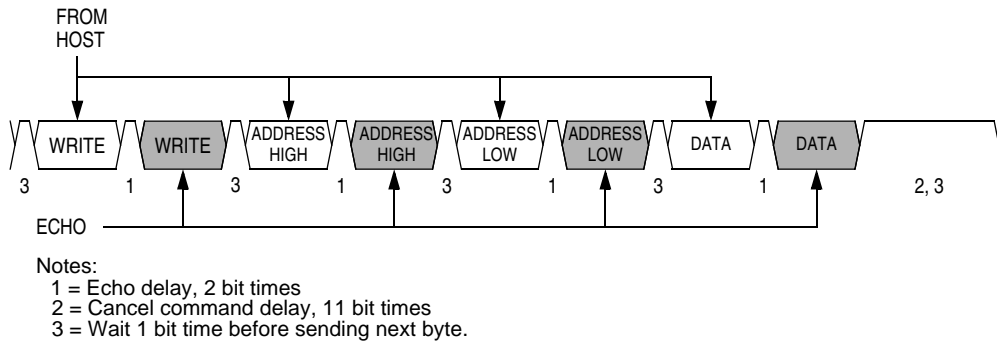
Figure 15-17. Write Transaction
