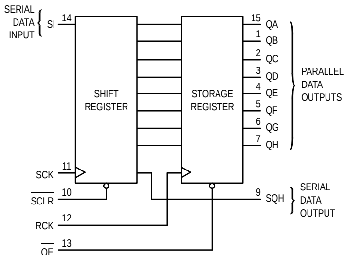
LOGIC DIAGRAM
