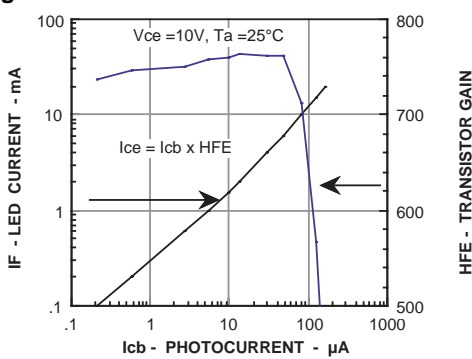
Figure 13. Transfer curve
