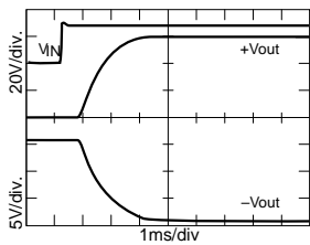
MFLHP2815D Turn On Response
