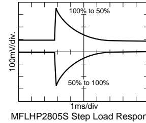
MFLHP2805S Step Load Response
