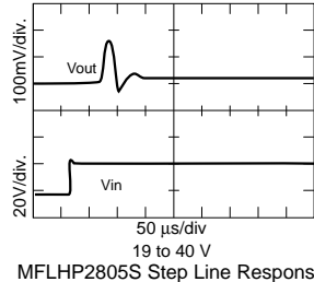
MFLHP2805S Step Line Response
