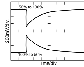
MFLHP2815D Step Load Response
