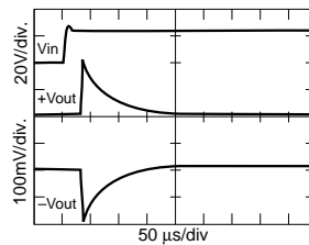
MFLHP2815D Step Line Response
