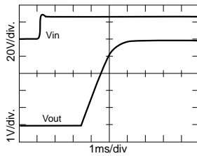
MFLHP2805S Turn On Response
