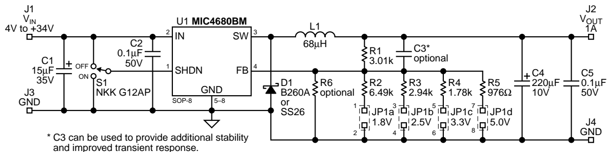
Figure 6a. Evaluation Board Schematic Diagram
