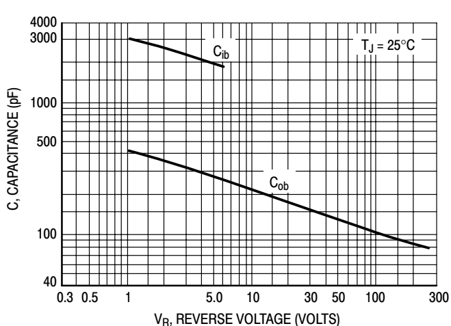
Figure 2. Capacitances
