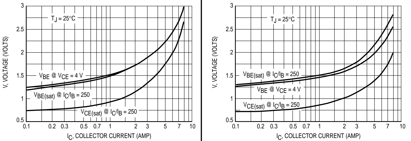
Figure 4. "On" Voltages
