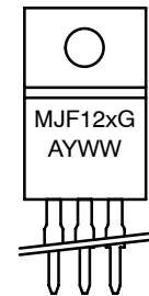
TO-220 CASE 221D-02 STYLE 2
