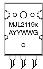
TO-3PBL (TO-264) CASE 340G
