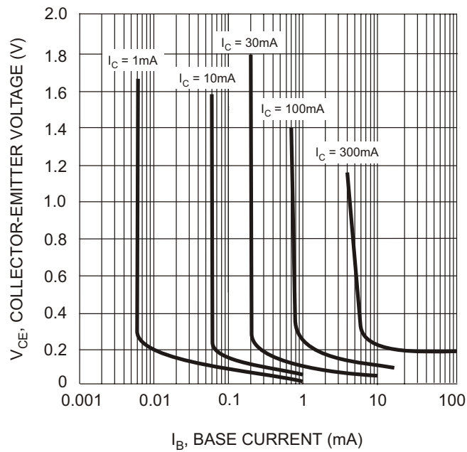
Fig. 3 Typical Collector Saturation Region
