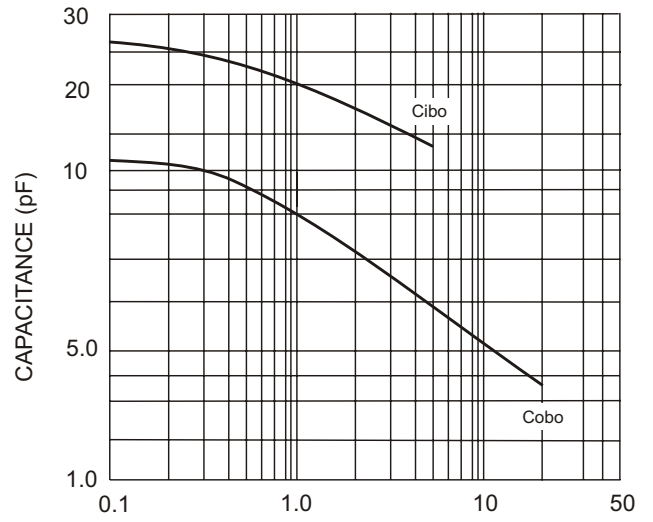
Fig. 2 Capacitances (Typical)
