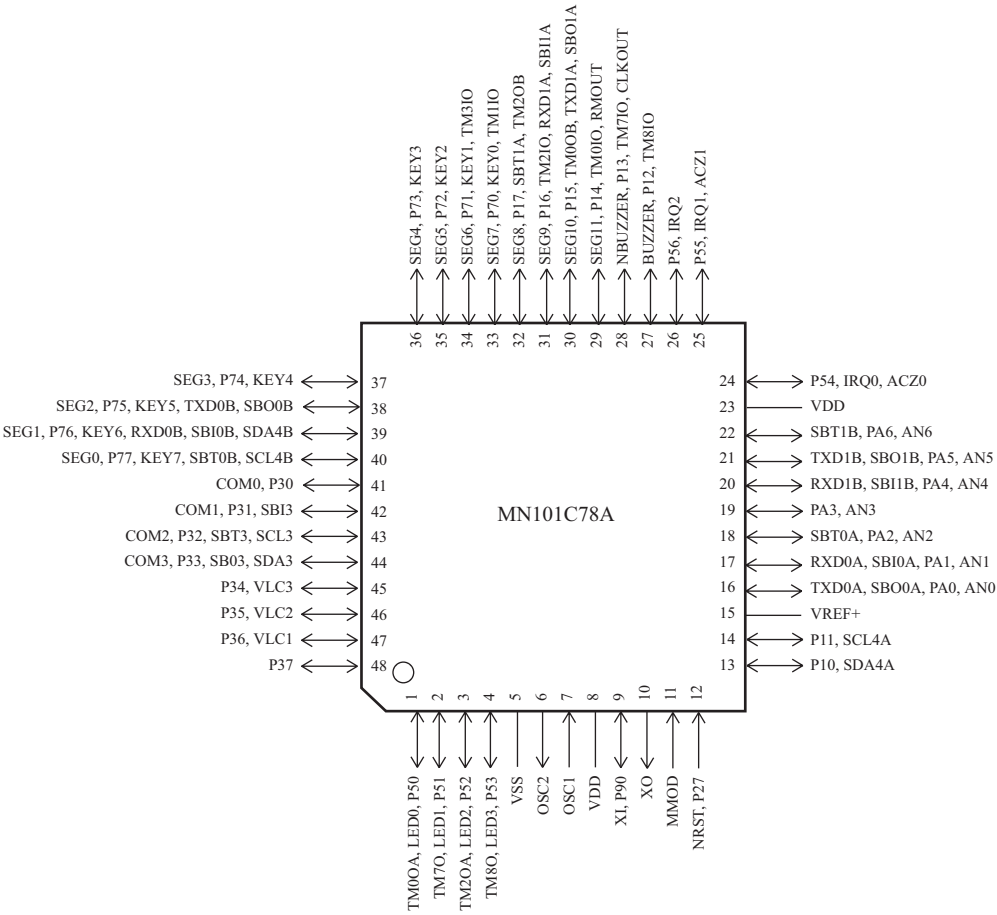
TQFP048-P-0707B
