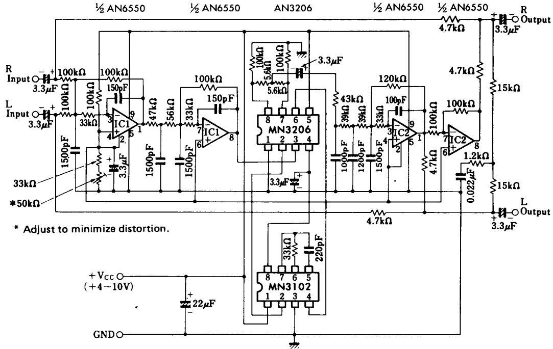
Vibrato and/or chorus effects Generation Circuit
