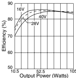
MOR289R5D Efficiency FIGURE 23
