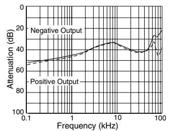
MOR2815D Audio Rejection FIGURE 28
