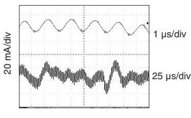
80% load each output MOR2805D Input Ripple (lin) FIGURE 42
