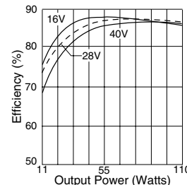
MOR2812D Efficiency FIGURE 24
