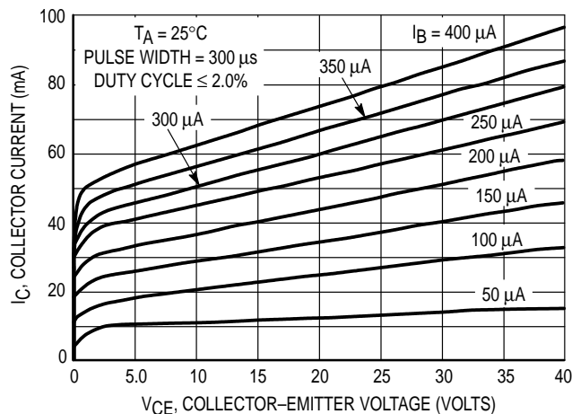
Figure 8. Collector Characteristics
