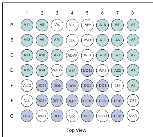
Figure 1: 56-Ball VFBGA
