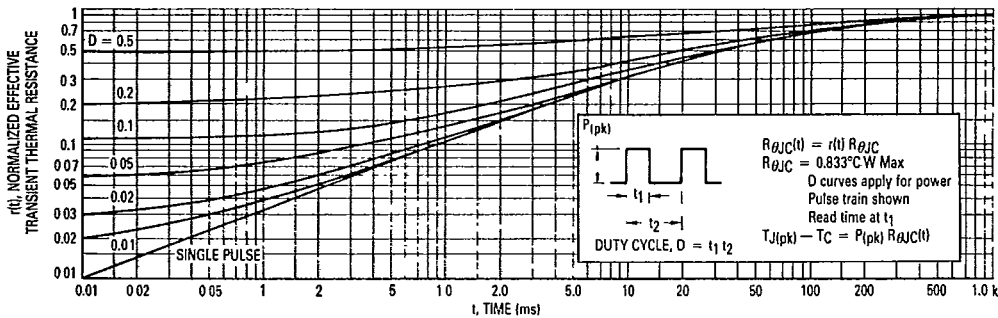
Figure 10. Thermal Response
