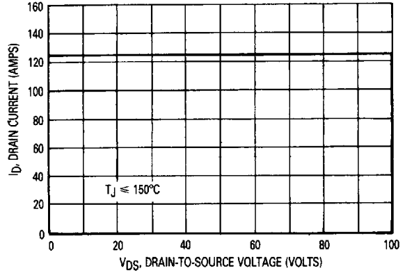
Figure 8. Maximum Rated Switching Safe Operating Area
