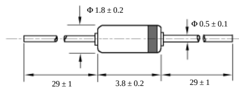
DO-35 (mm)
