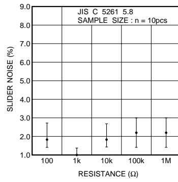
Fig.14 Wiper noise
