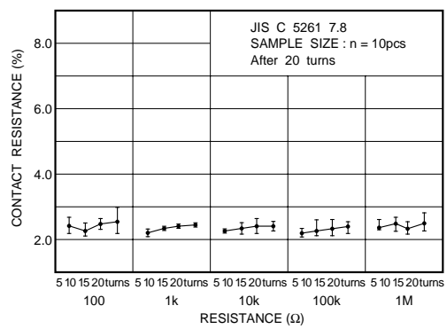
Fig.6-2 Endurance (wiper)
