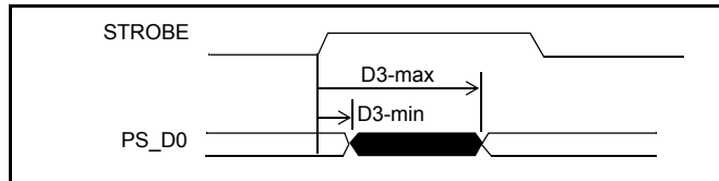
Figure 25 - Serial Interface Output Delay Timing
