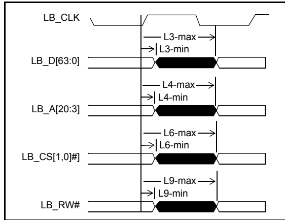
Figure 10 - Local Memory Interface - Output valid delay timing
