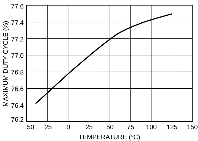
Figure 9. Maximum Duty Cycle versus Temperature
