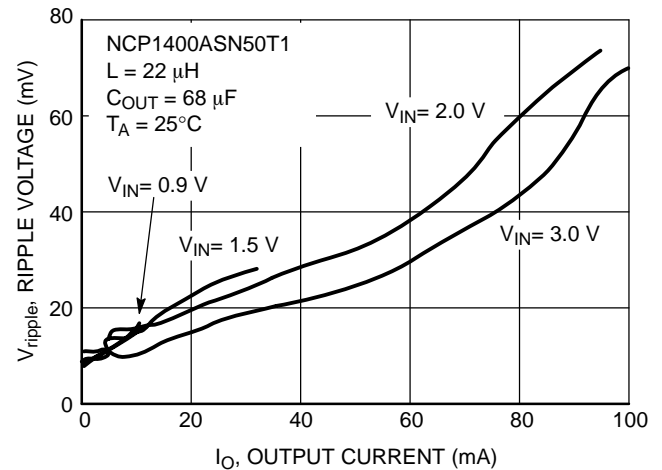
Figure 31. NCP1400ASN50T1 Ripple Voltage vs. Output Current
