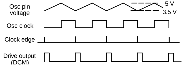
Figure 37. Oscillator Mode Timing Diagram in DCM
