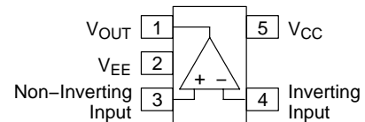
Style 2 Pinout (SN2T1, SQ2T1)
