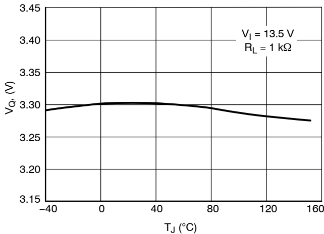
Figure 10. Output Voltage V_Q vs. Junction Temperature T_J , 3.3 V Version
