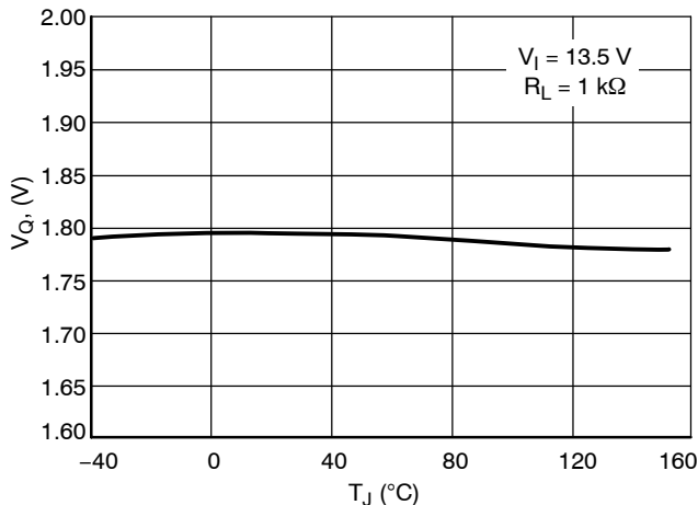
Figure 8. Output Voltage V_Q vs. Junction Temperature T_J , 1.8 V Version
