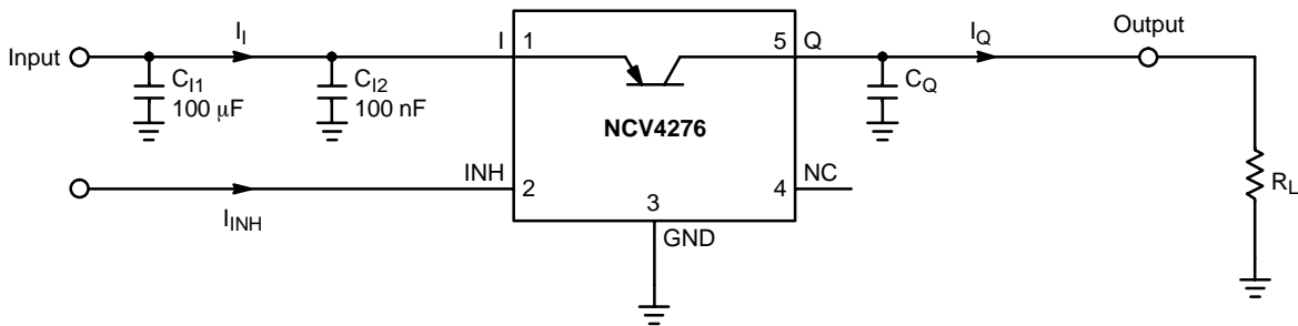
Figure 2. Measuring Circuit
