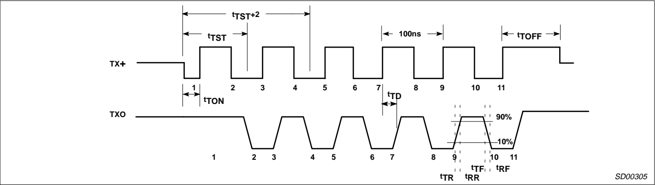
Figure 5. Transmitter Timing
