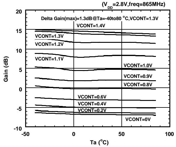
Gain vs. Ta (Variable VCONT)
