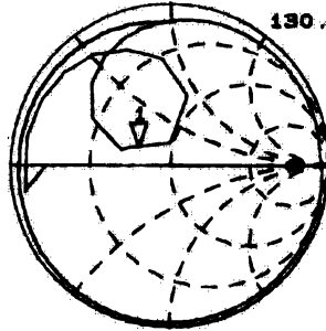
IFOUT PORT EXTERNAL MATCHING NETWORK IMPEDANCE PLOT
