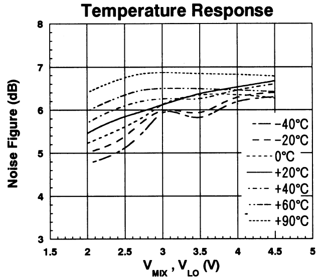
Noise Figure vs. V_{MIX} , V_{LO}
