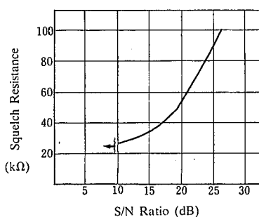
Graph 20 Squelch Sensitivity Characteristics
